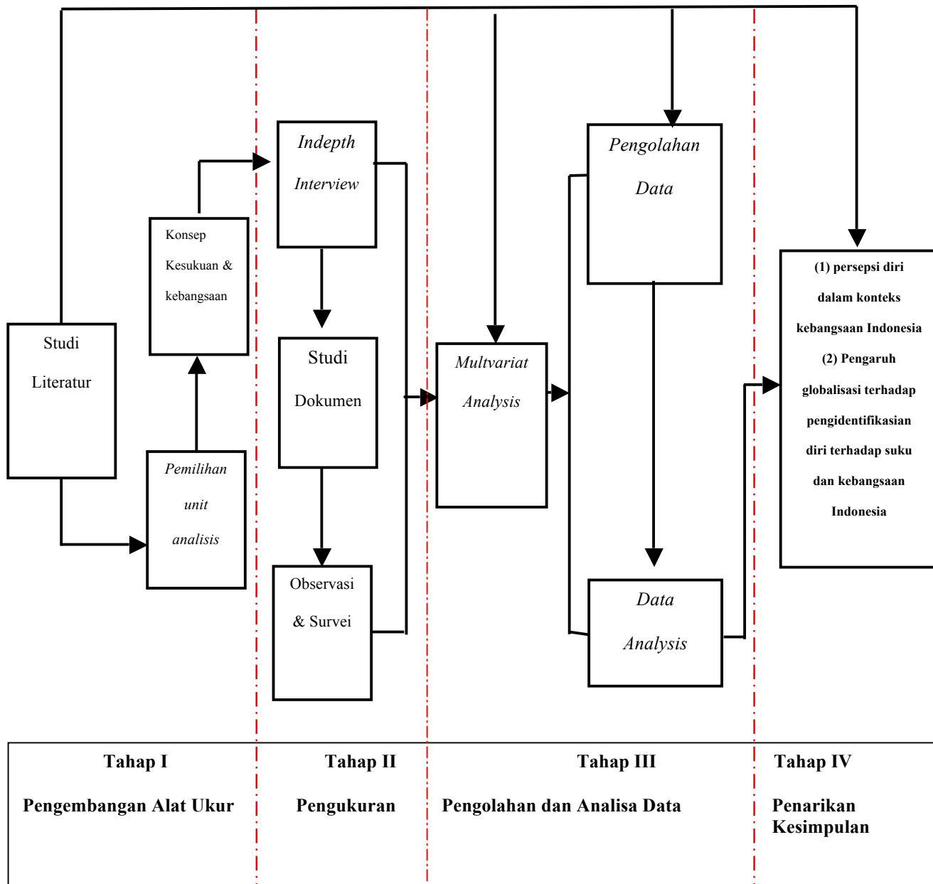
Gambar 2. Roadmap Penelitian
