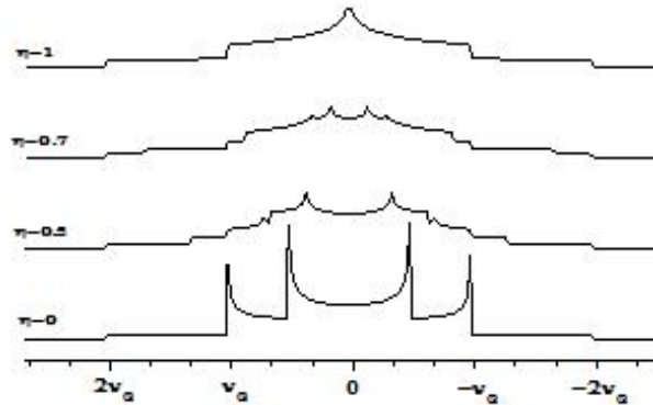
Figure 6. The quadrupole perturbed powder patterns for an I=3/2 nucleus showing the outer satellite transitions to first-order where \nu_Q = (3\chi_Q)/(2I(2I - 1)) .
