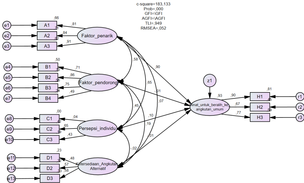
Gambar 4. Hasil Estimasi Metode Asymptotically Distribution Free (ADF)
