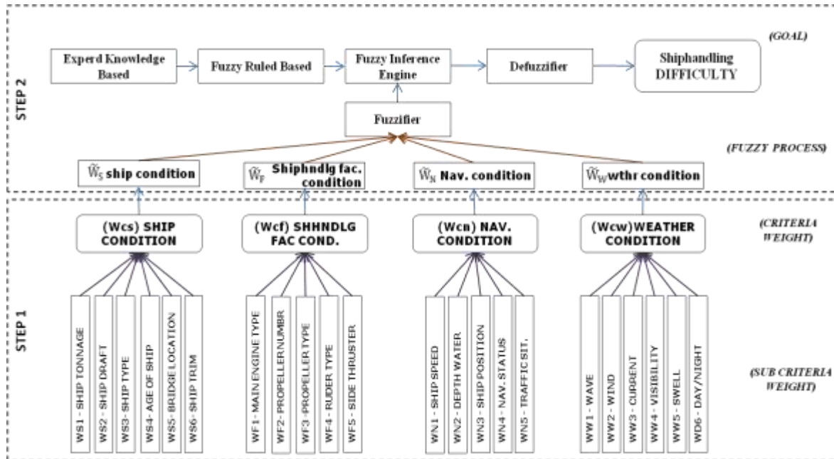
Figure 1 Shiphandling Difficulty Model for Ferry Framework
