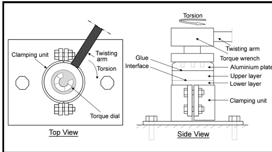
Figure 1 Schematic Diagram of the Laboratory Based Manual Torque Bond Test Developed by Choi Et Al (2005)
