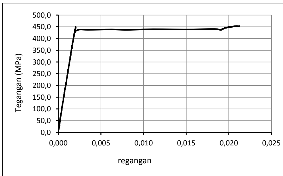
Gambar 4.5 Kurva tegangan – regangan specimen B2
