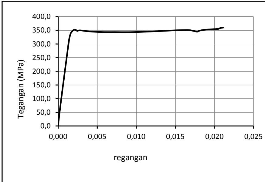
Gambar 4.2 Kurva tegangan – regangan specimen A2
