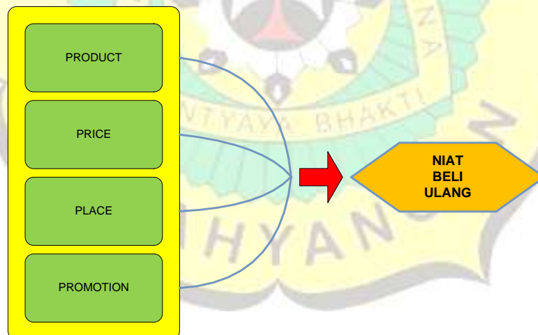
Gambar 3 Model Penelitian
